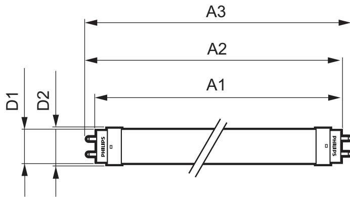
MASTER LEDtube SA3 600mm 850lm 856 G13
